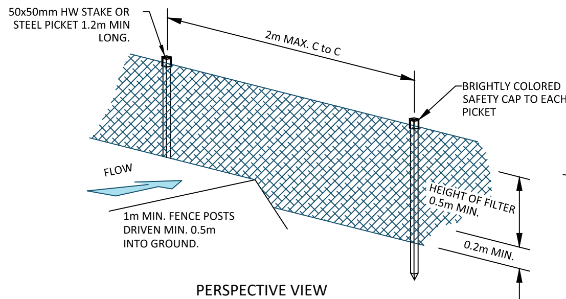
SEDIMENT FENCE DETAIL
